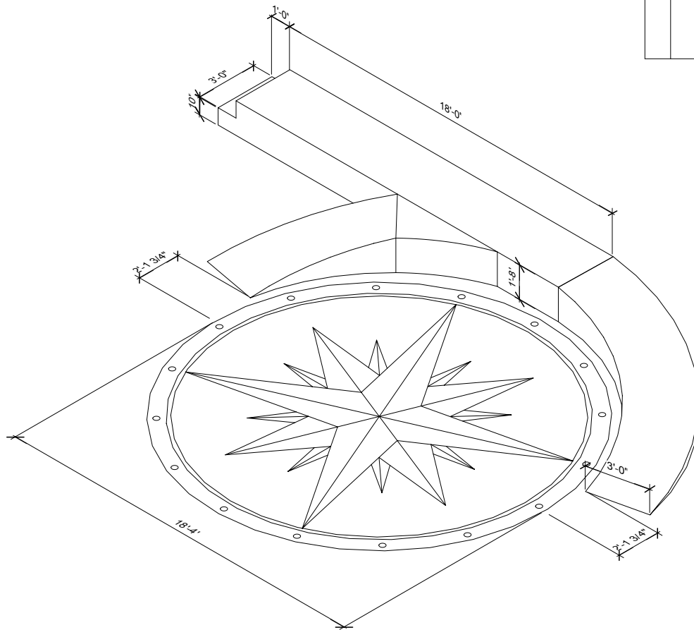
Right Isometric
